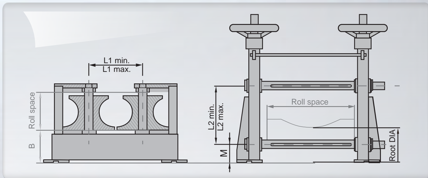
Support vertical
