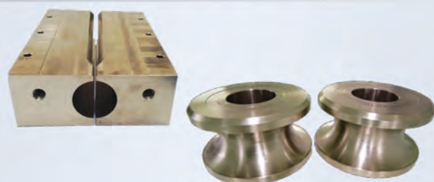
Rohrformen AMPCO® 18/21/22/25
